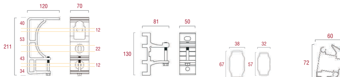
supporto universale universal fixing bracket
